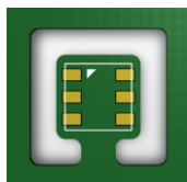
Figure 10 The top view of AHT20 printed circuit board, the design of the milling slit is added in the figure, The heat transfer can be reduced to a minimum.
