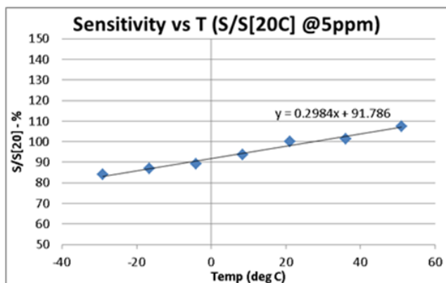
Effect of Temperature on Sensitivity
