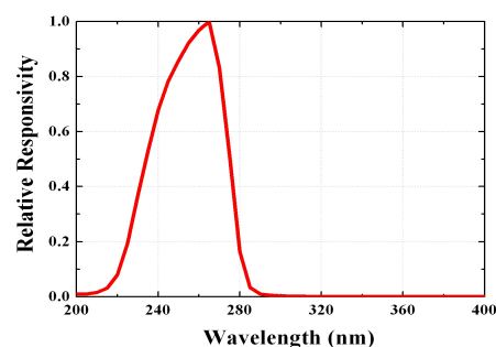
Fig. 2 Responsivity Curve
