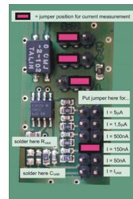
Jumper positions for photodiode input
