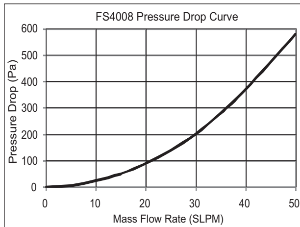
Figure 1.4: FS4008 pressure drop v.s. flow rate.
