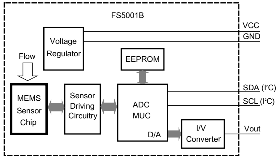
Functional block diagram of the FS5001B.
