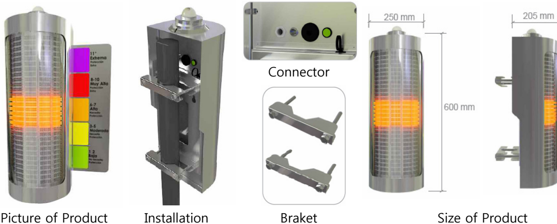
Fig1. Physical Dimentions
