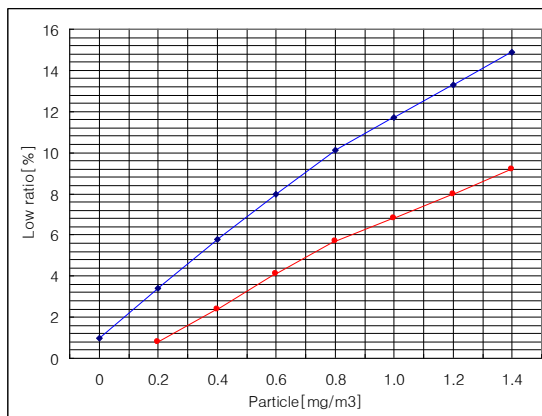
Fig. -2. Sensor Characteristics vs Low ratio
