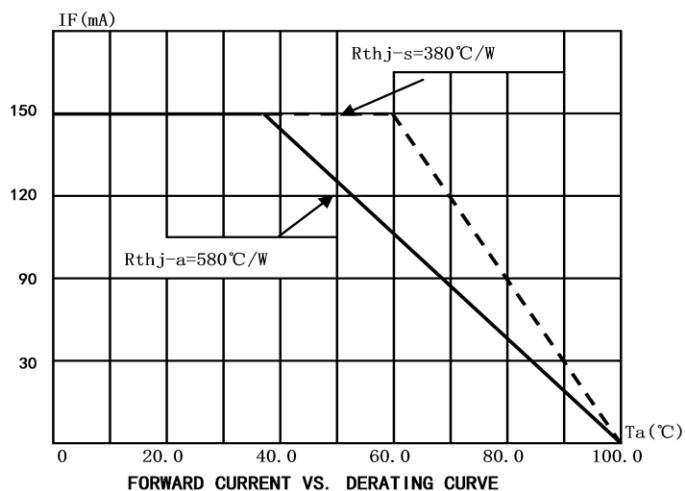
FORWARD CURRENT VS. DERATING CURVE
