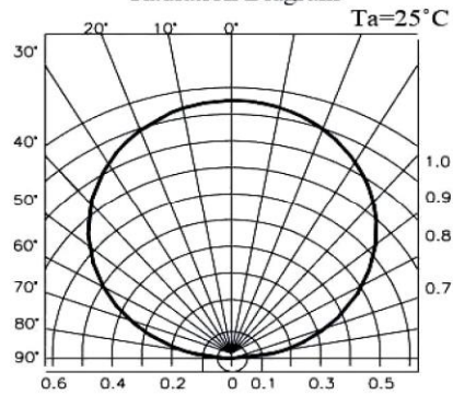
Radiation Diagram
