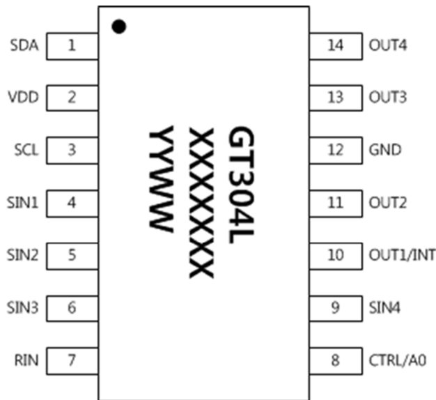
Figure 4.1 SOP14L Pinout Diagram (Top View)
