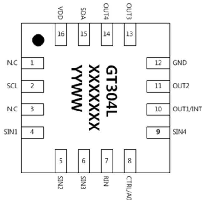
Figure 4.2 QFN16L Pinout Diagram (Top View)
