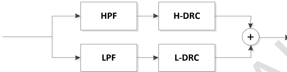
Figure 19. Block Diagram of Dynamic Range Control
