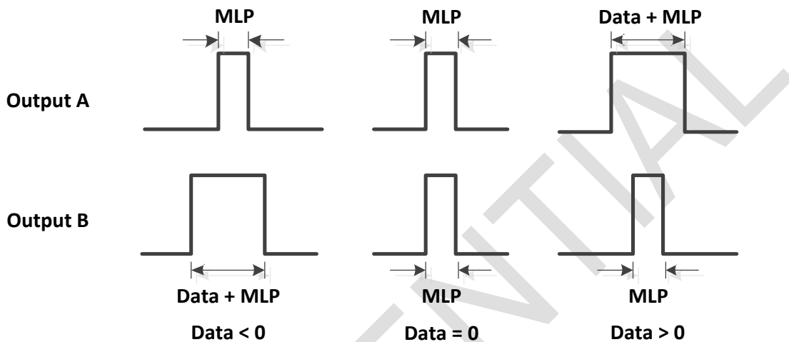
Figure 17. Compensation by MLP
