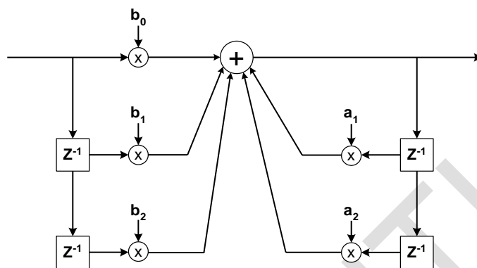
Figure 13. Bi-Quad Filter Structure
