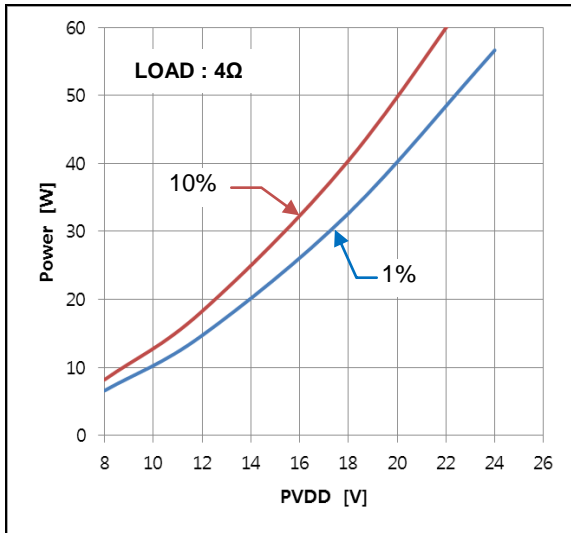
Output Power vs. PVDD
