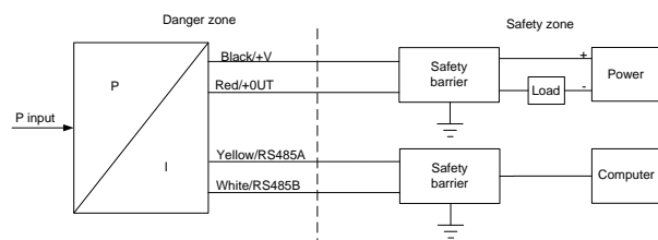
C: This Ann explosion-proof type electrical connection methods are shown below:
