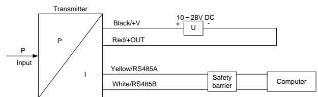
C: This Ann explosion-proof type electrical connection methods are shown below:
